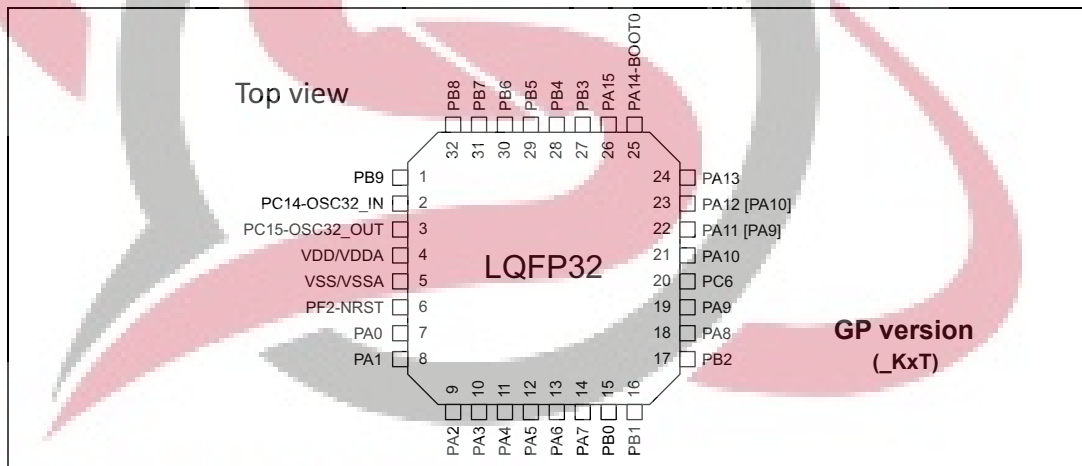
Figure 7. STM32G071KxT LQFP32 pinout
